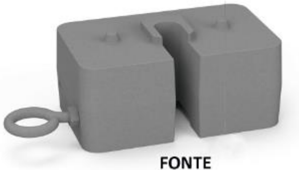
235*145*100h 22kg Passage 26 mm Ref. CE037
