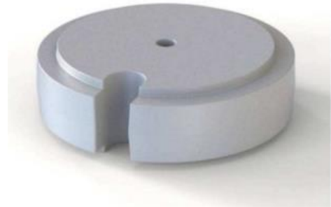
Diameter 300*88h 40kg Durchgang 18 mm Loch 18 mm Ref. GALD300H88
